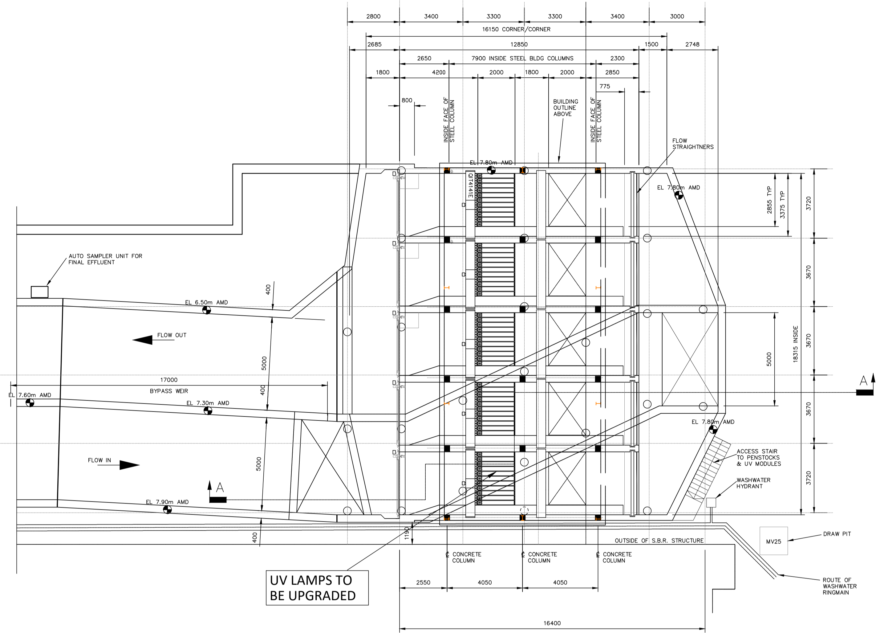
PLAN
