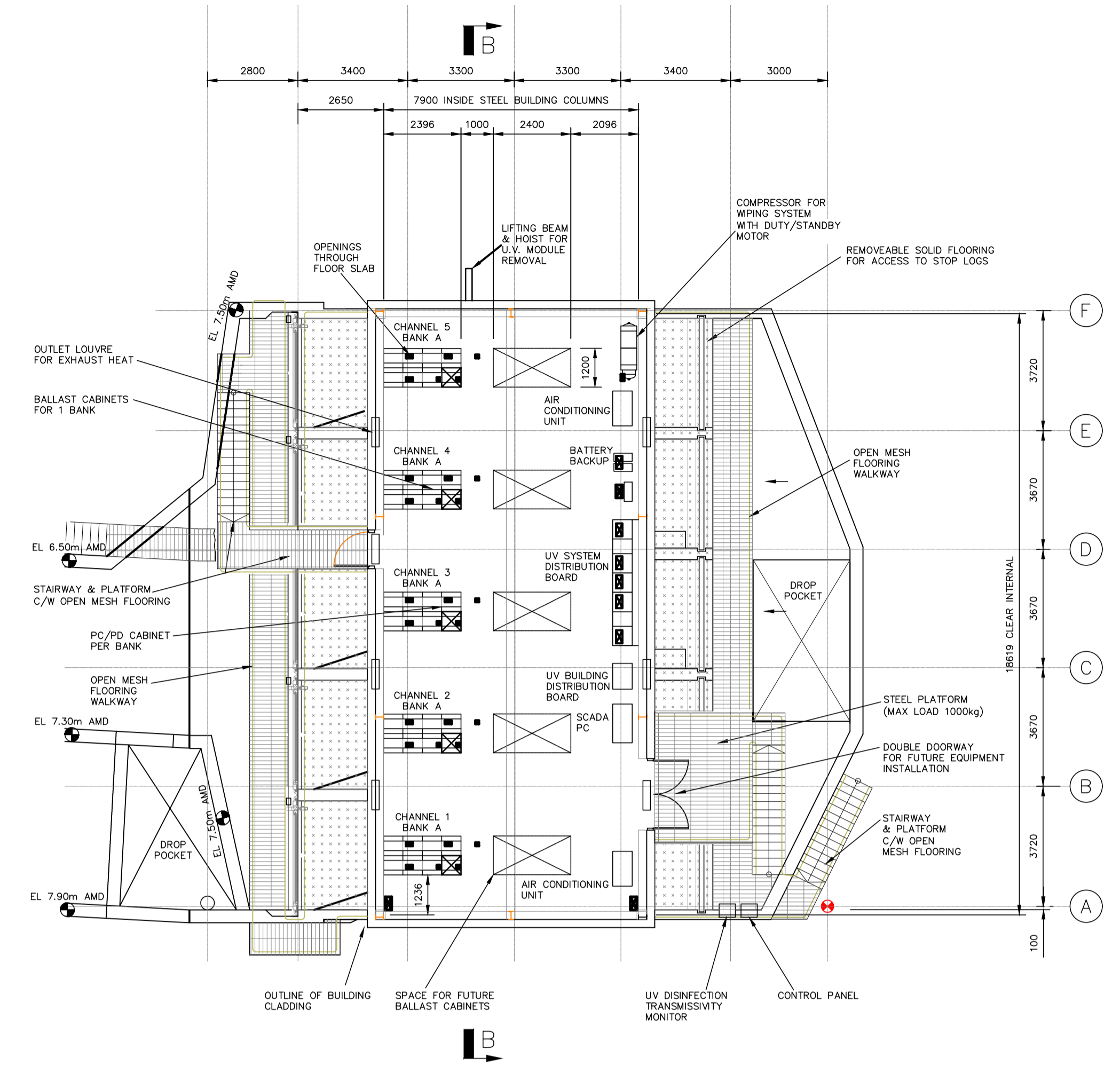
UPPER FLOOR PLAN
