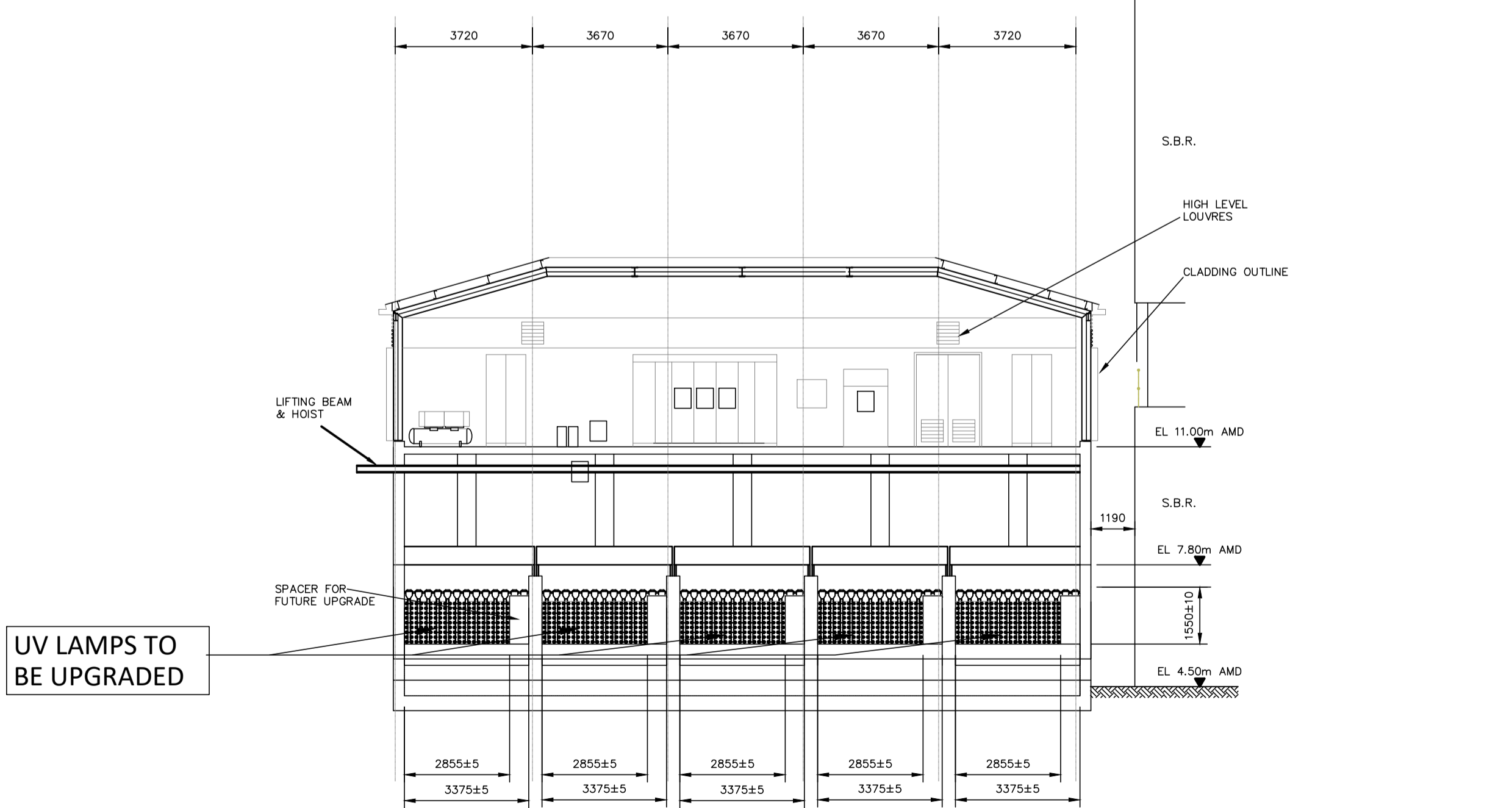
SECTION B-B
